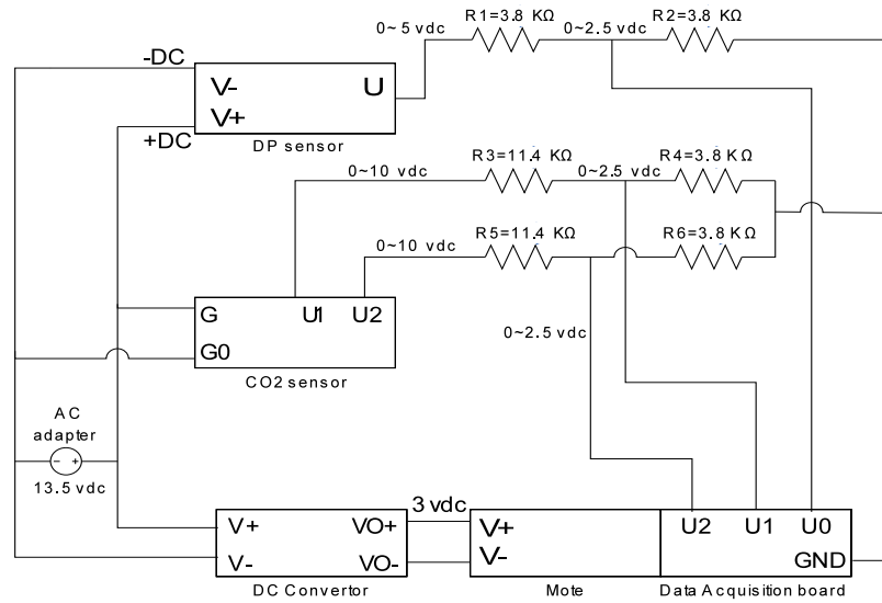
Figure 5.9: Wireless sensor package wiring diagram
