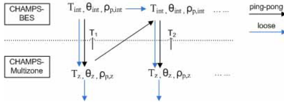
Figure 4.1: CHAMPS-Multizone and CHAMPS-BES Integration Methods
